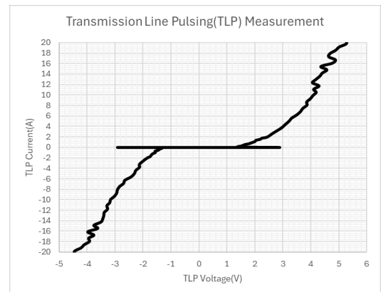
Figure 4. TLP (1/100ns)
